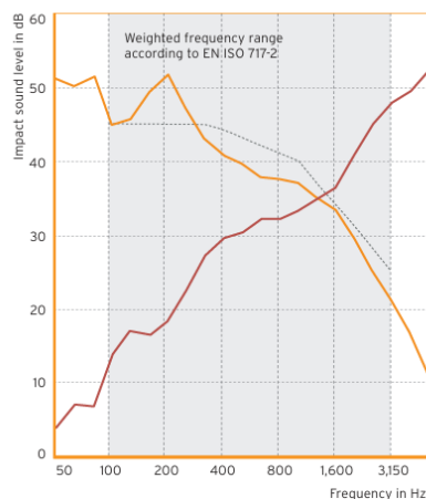
Impact sound insulation according to EN ISO 10140-3
