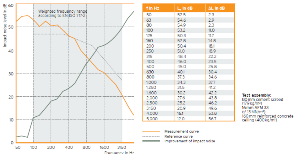
Impact noise improvement level according to EN ISO 10140-3
