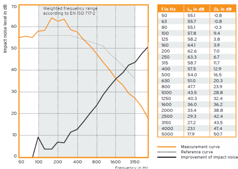
Impact noise improvement level according to EN ISO 10140-3
